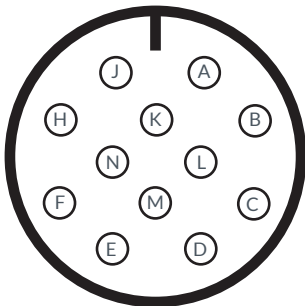
PIN PINOUT
