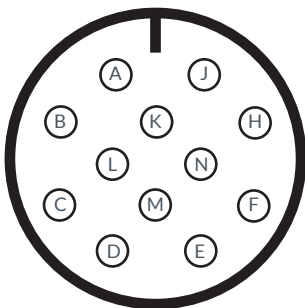
SOCKET PINOUT
